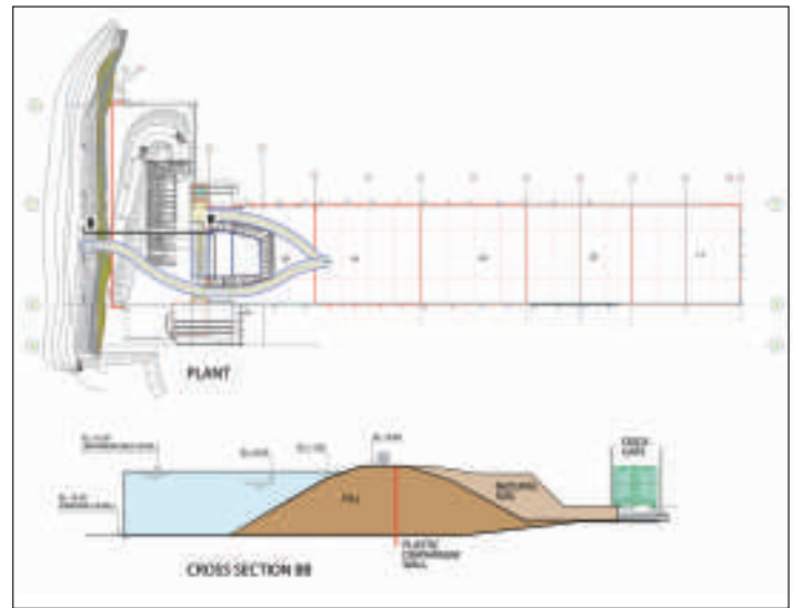
Figure 5: Cofferdam
